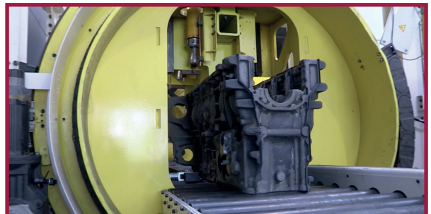
Rotating decorating station with hammering* (0 to 180°)
